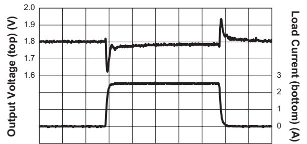
Time (100μs/div)
