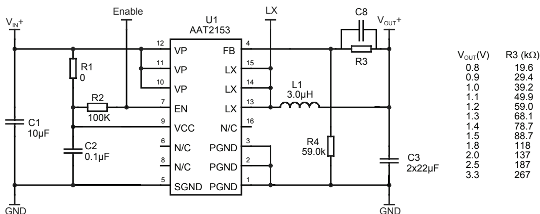
C1 Murata 10µF 6.3V X5R GRM42-6X5R106K6.3 C3 Murata 22µF 6.3V GRM21BR60J226ME39L X5R 0805 L1 see Table 2 R1 and C2 are an optional noise filter for internal V CC . R6, C4, C5-C7 are not populated C8 100pF to 1nF feed-forward capacitor for enhanced transient response
